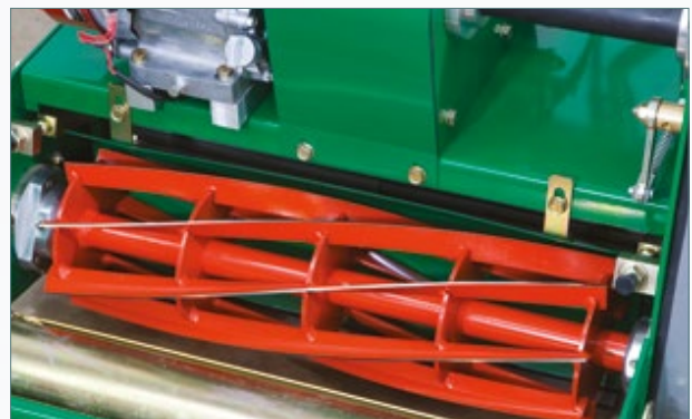
Choice of two cutting widths with 5 and 7 blade options
