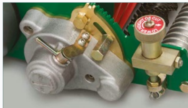
Simple to operate groomer drive engagement
