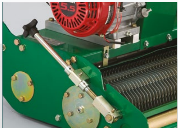
Simple tool free height of operation adjustment
